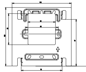
② FRONT VIEW:WALL MOUNTING BRACKET PLACEMENT
